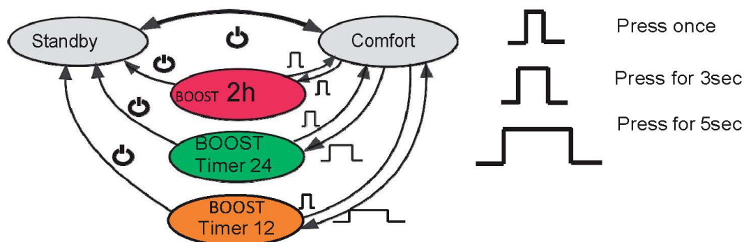
Functional diagram
